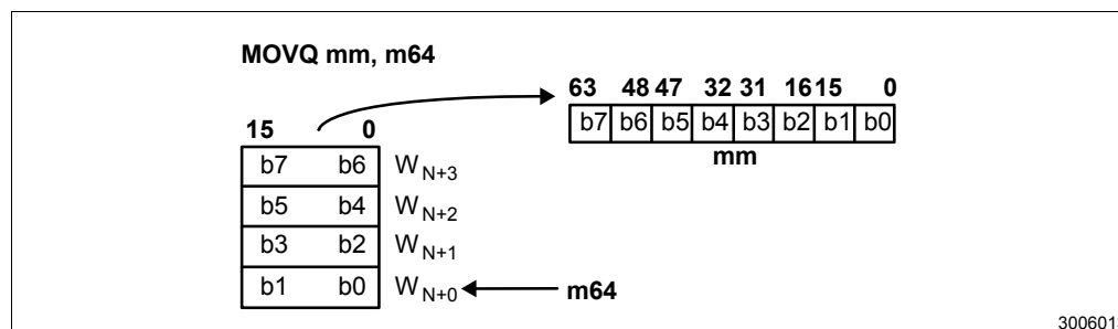
Figure 3-2. Operation of the MOVQ Instruction
